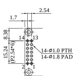
PIN DETAIL
