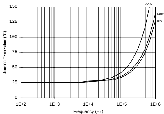
Figure 34. IR2112S T_J vs. Frequency (IRFBC40) R_{\text{GATE}} = 15\Omega , V_{\text{CC}} = 15\text{V}
