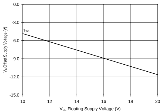
Figure 36. Maximum V_S Negative Offset vs. V_{\text{BS}} Supply Voltage
