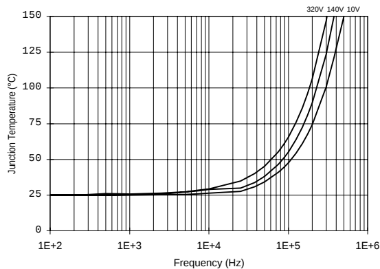
Figure 35. IR2112S T_J vs. Frequency (IRFPE50) R_{\text{GATE}} = 10\Omega , V_{\text{CC}} = 15\text{V}
