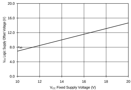
Figure 37. Maximum V_{\text{SS}} Positive Offset vs. V_{\text{CC}} Supply Voltage
